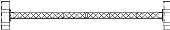
Single span truss rigid restrained at both ends
