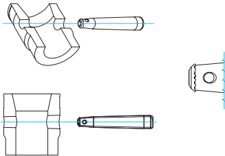
Deformation of the conical pins
