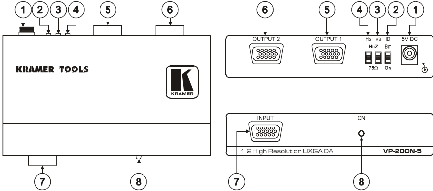
Figure 1: VP-200N-5 1:2 High Resolution UXGA DA
