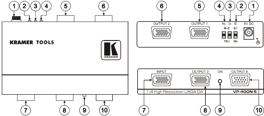
Figure 3: VP-400N-5 1:4 High Resolution UXGA DA
