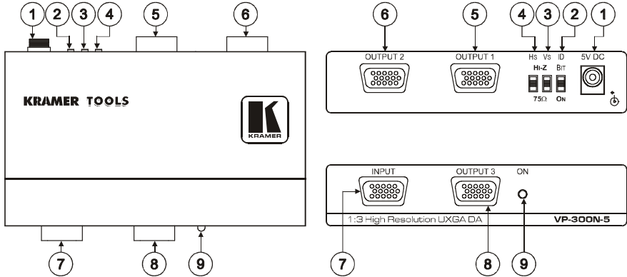
Figure 2: VP-300N-5 1:3 High Resolution UXGA DA
