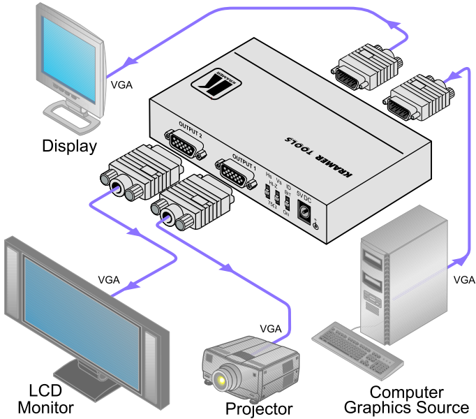
Figure 4: Connecting the VP-300N-5 1:3 High Resolution UXGA DA
