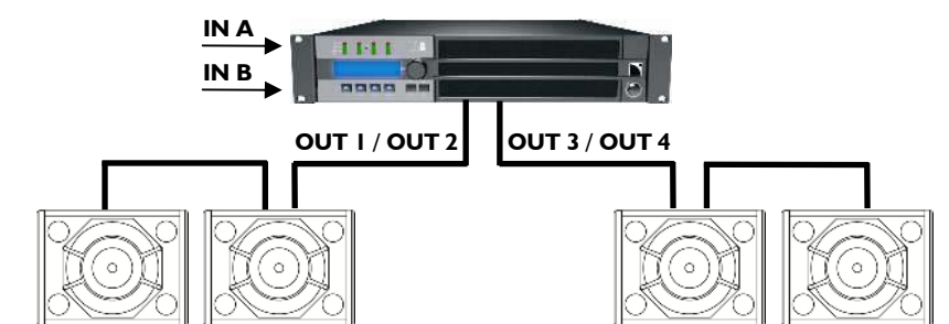
Figure 7: Four I15XT HiQ enclosures connected to an LA8 controller
