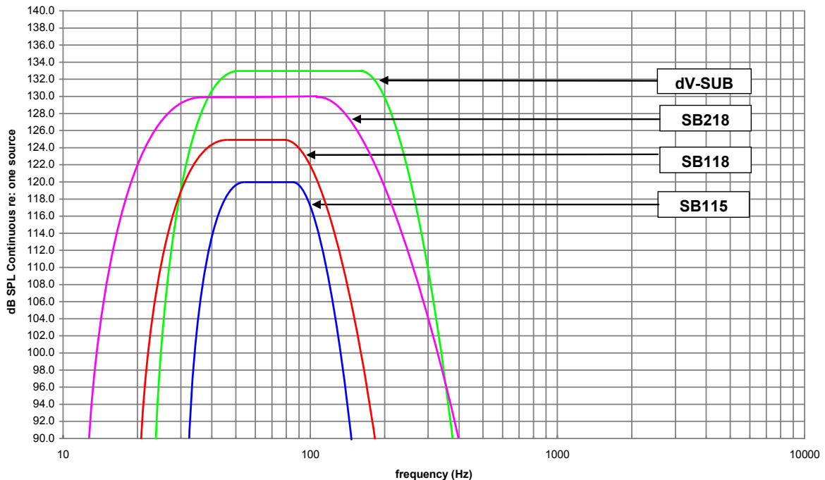
Figure 40: L-ACOUSTICS Subwoofer Continuous Unweighted SPL Comparison
