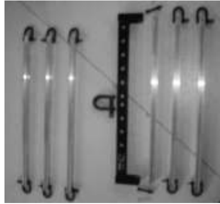
(2) Close up detail of rigging accessories (6 ARCOUPL, 1 BUMP3 plus shackles)
