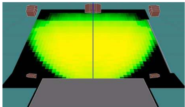
Centre Cluster A-Weighted SPL Map
