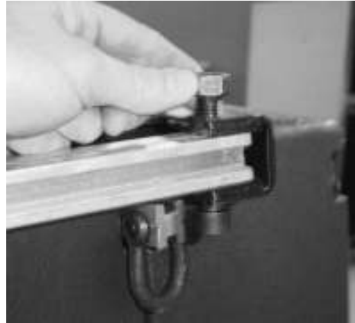
(10) ARCOUPL attached to the main body of the LIFTBAR at the rear
