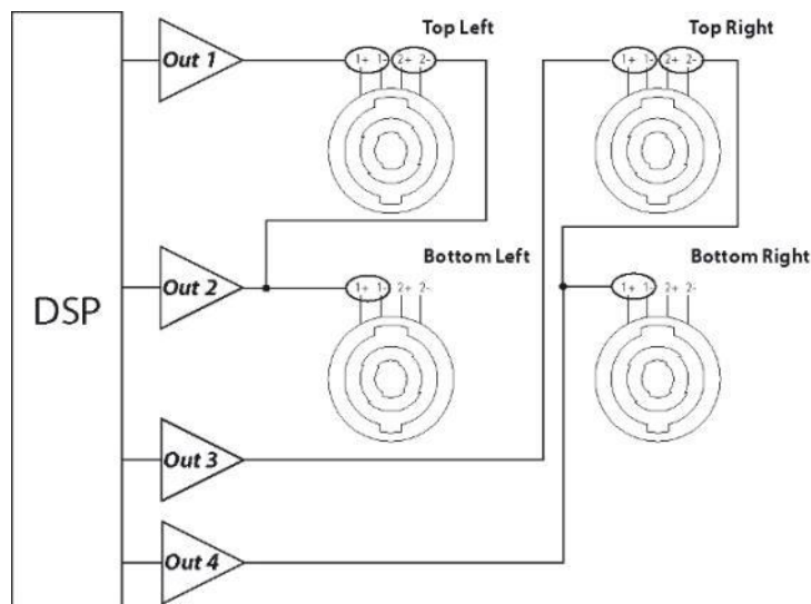
Figure 10: Output audio paths
