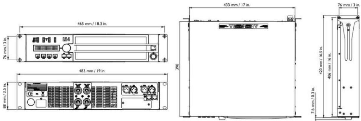
Figure 5: LA4 dimensions
