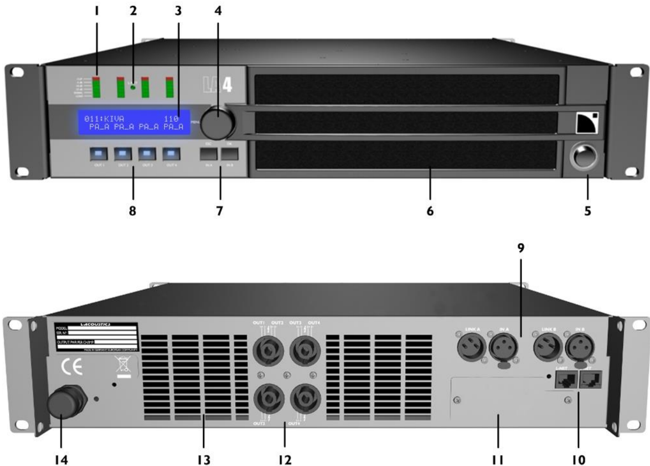
Figure 2: LA4 front and rear panels
