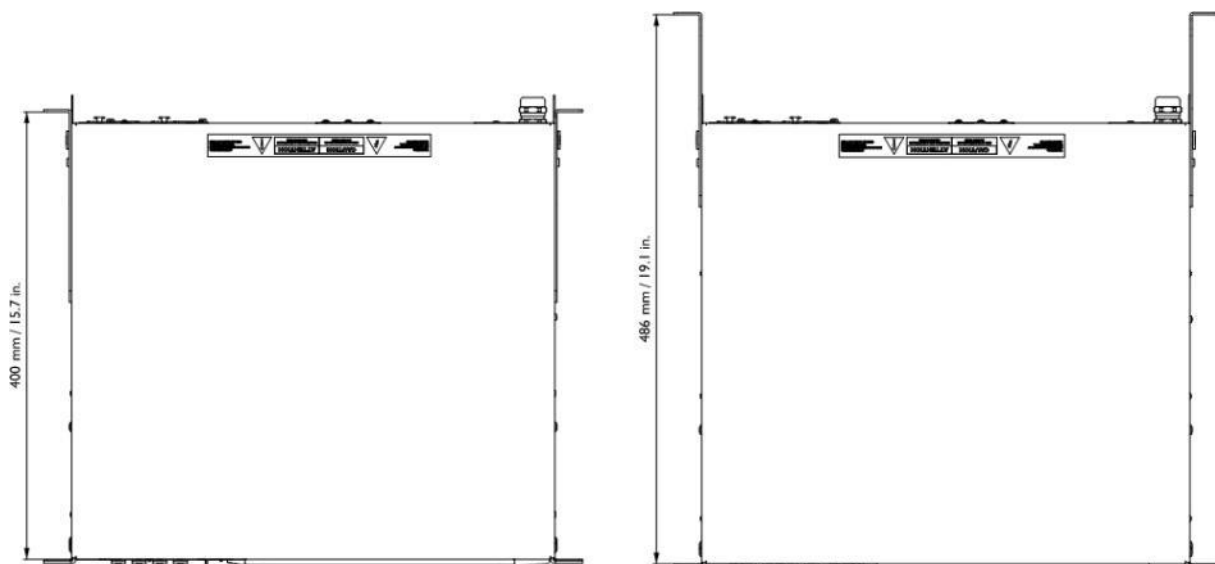
Figure 6: LA4 with rear rack support brackets
