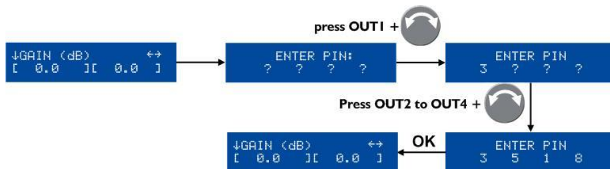
Figure 22: Entering a PIN code
