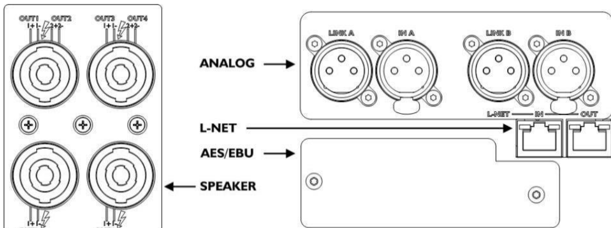
Figure 7: LA4 rear connection panels
