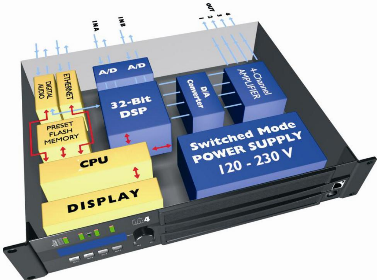
Figure 3: LA4 simplified block diagram
