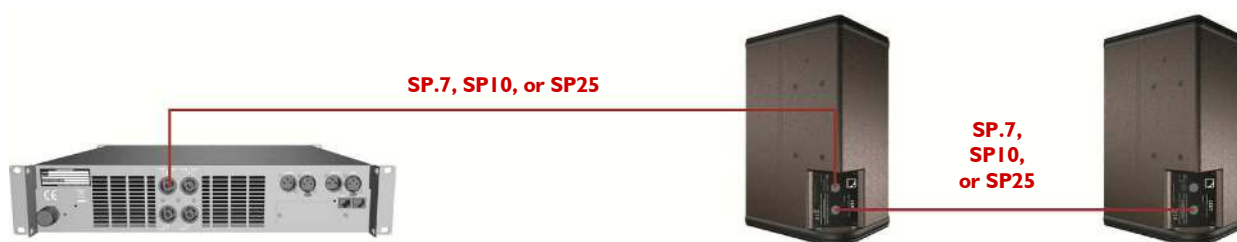
Figure 5: Connecting two ACTIVE I2XT in parallel to the channel 1 of an LA4 / LA4X controller
